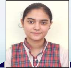
HIMANSHI 93.6%
